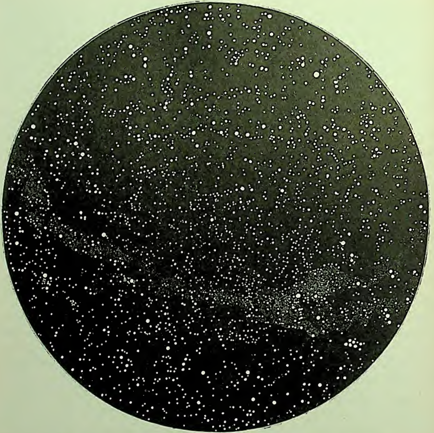
Figure 11. The stars visible to the naked eye in the northern celestial hemisphere.
