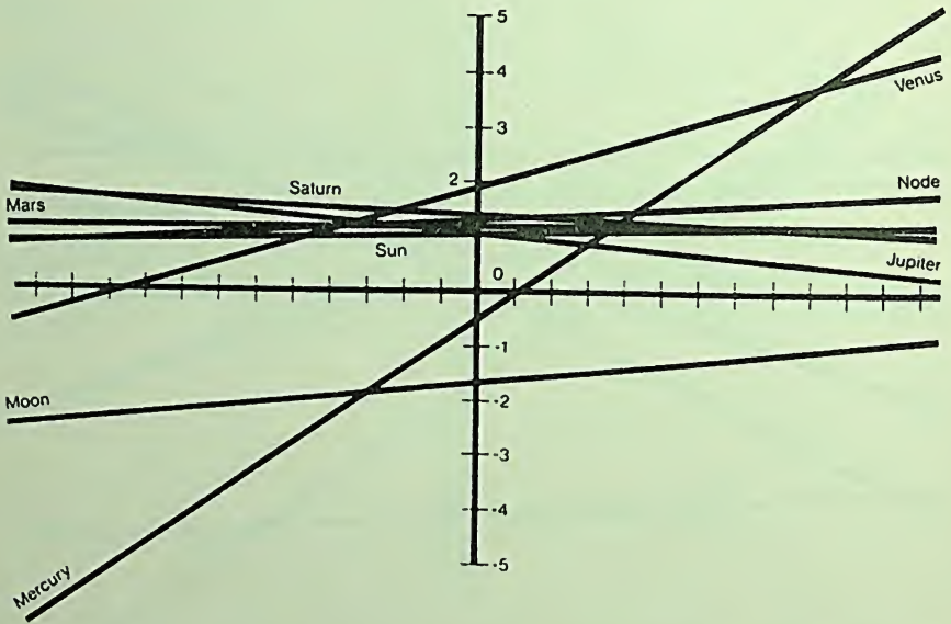
Figure A2.3 A comparison between Ptolemy's system and modern astronomy. The horizontal axis represents time in units of 40 years. The origin corresponds to Jan. 1, A.D. 161, a date in Ptolemy's lifetime. The vertical axis represents the difference in degrees between modern mean planetary positions and Ptolemy's mean planetary positions. Both the modern and the Ptolemaic mean longitudes are relative to Zeta Piscium (using modern and Ptolemaic calculations for Zeta Piscium, respectively). The differences are plotted for the seven planets and the ascending node of the moon. Ptolemy does fairly well for the sun, Mars, Saturn, Jupiter, and the ascending node, although he does make a systematic error for these planets. A much greater difference arises between Ptolemaic and modern calculations if they are both made relative to the vernal equinox. This suggests that Ptolemy's observations were initially made relative to a fixed star, and then converted to the tropical Zodiac.
