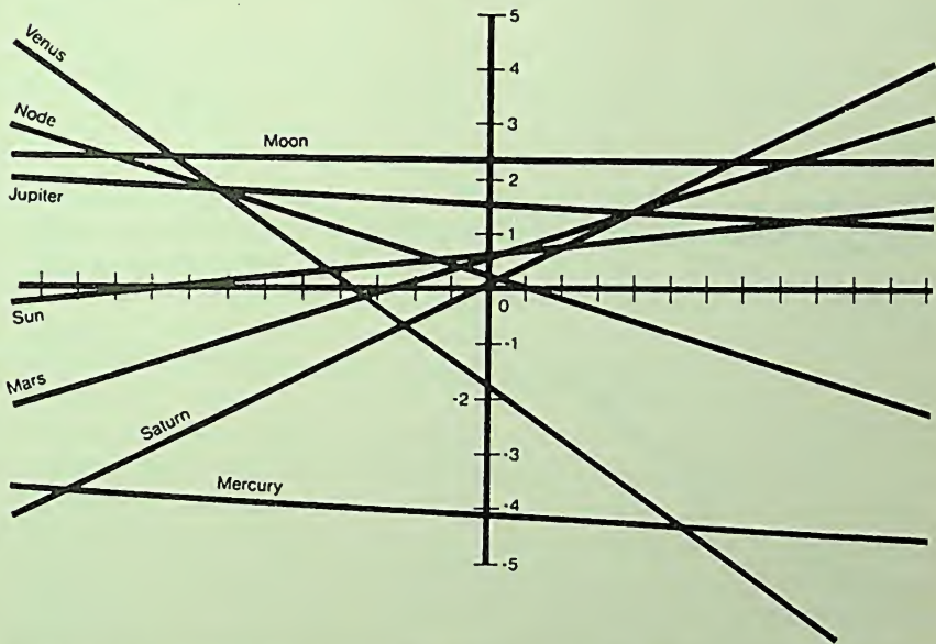
Figure A2.2 A comparison between Āryabhaṭa's system and Ptolemaic astronomy. The horizontal axis represents time in units of 40 years. The origin corresponds to noon on Mar. 21, A.D. 499. The vertical axis represents the difference in degrees between Ptolemy's mean planetary positions relative to Zeta Piscium and Āryabhaṭa's mean planetary positions. These differences are plotted for the seven planets and Rāhu (the ascending node of the moon). In this case there is a sharp convergence only for the sun, Mars, Saturn, and the ascending node. This figure should be compared with Figure A2.1.
