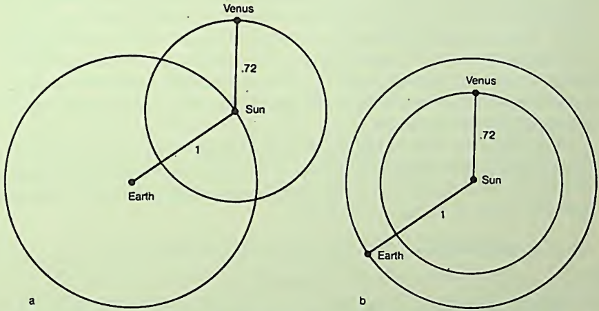
Figure 1. The geocentric and heliocentric models of the motion of Venus: a) the geocentric model of the Sūrya-siddhānta ; b) the heliocentric model.
