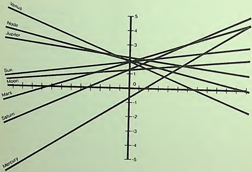
Figure A2.1 Comparison between Āryabhaṭa's system and modern astronomy. The horizontal axis represents time in units of 40 years. The origin corresponds to noon of Mar. 21, A.D. 499. The vertical axis represents the difference in degrees between modern mean planetary positions relative to Zeta Piscium and Āryabhaṭa's mean planetary positions. These differences are plotted for the seven planets and Rāhu (the ascending node of the moon). Note that for all planets except Mercury, the differences between Āryabhaṭa's calculations and modern calculations converge sharply at about A.D. 539.
