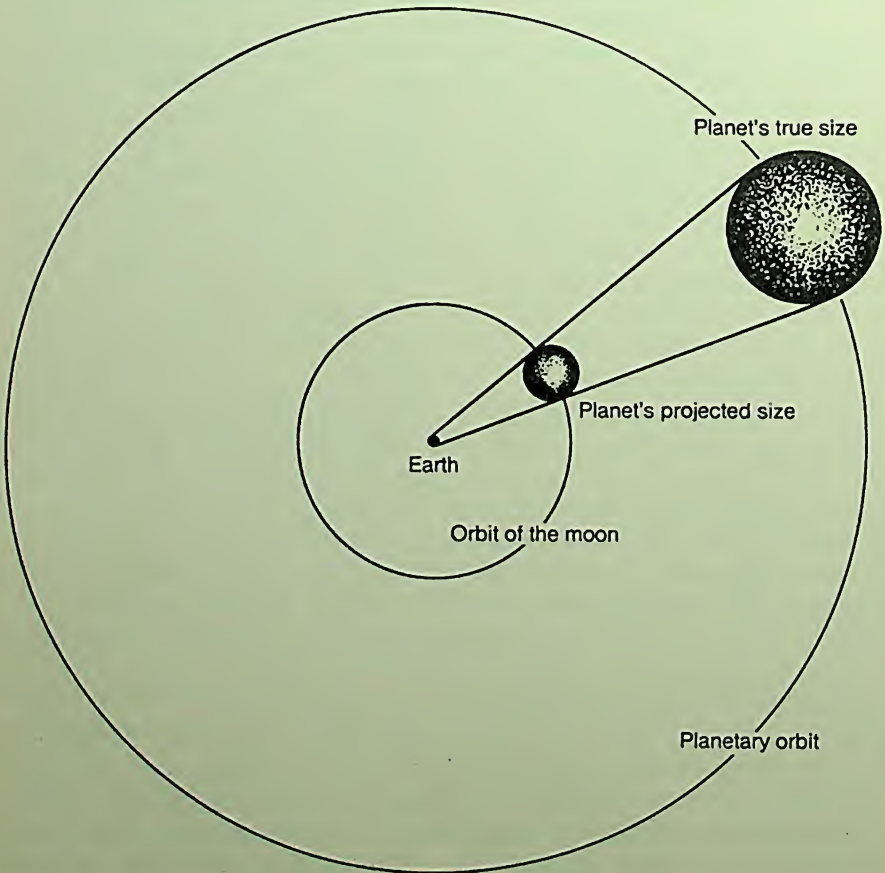
Figure 2. The relationship between the true diameter of a planet and its diameter projected to the orbit of the moon.
