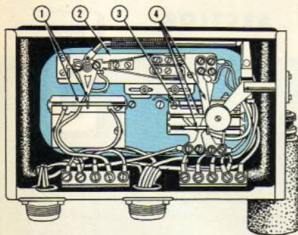
Stabilizer
