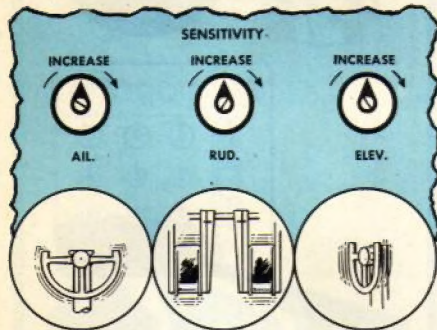
SENSITIVITY ADJUSTMENT
